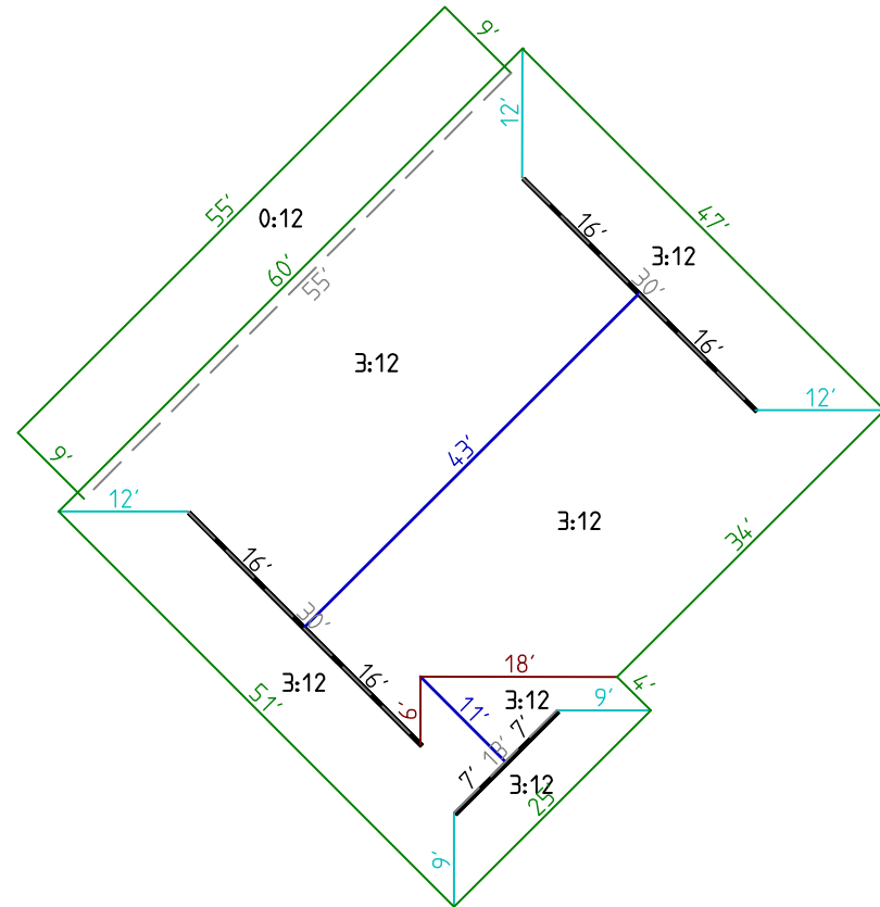
LENGTHS & PITCHES PLAN
